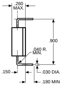
COMMON LEAD
