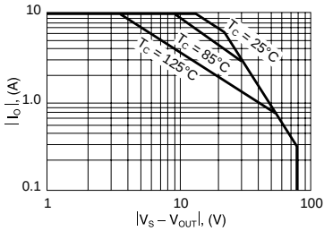
Copper Slug TO-3 Safe Operating Area OMA541SKC
