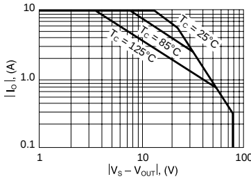
Standard TO-3 Safe Operating Area OMA541SK
