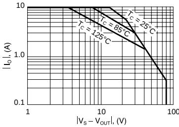
Power DIP Safe Operating Area OMA541SD/SDZ
