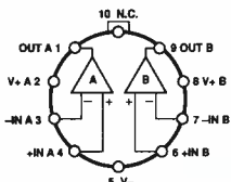
TO-100 (K-Suffix) OP-04
