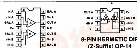
14-PIN HERMETIC DIP (Y-Suffix) OP-04
