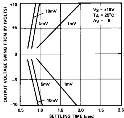
SETTLING TIME
