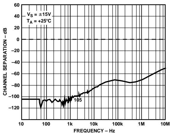
Figure 16. Channel Separation
