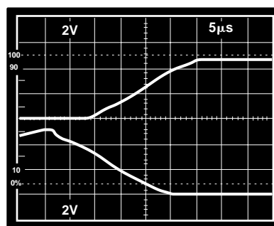
Figure 11. Precision Comparator
