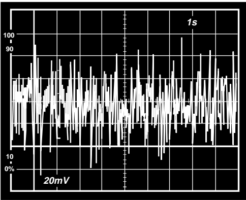
Figure 39. Input Voltage Noise @ ±15 V (20 nV/div)
