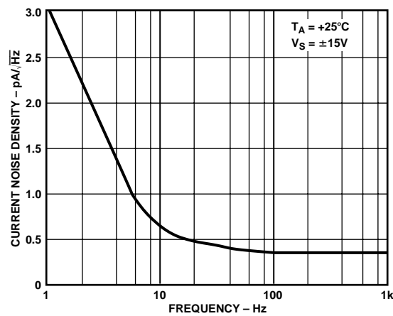
Figure 30. Current Noise Density vs. Frequency
