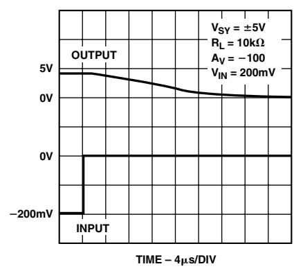
TPC 33. Negative Overtolerance Recovery
