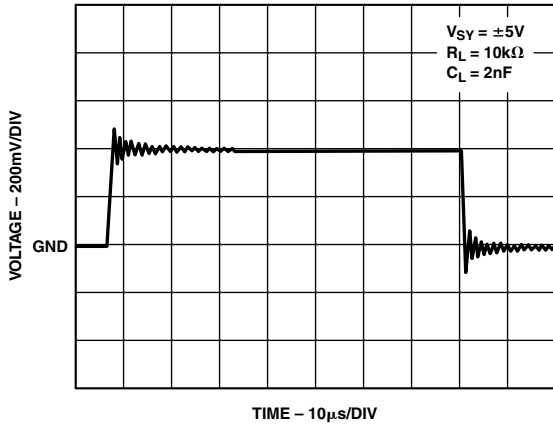
Figure 6. Capacitive Load Drive without Snubber
