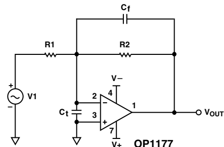
Figure 10. Compensation Using Feedback Capacitor
