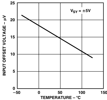
TPC 41. |V_{0s}| vs. Temperature
