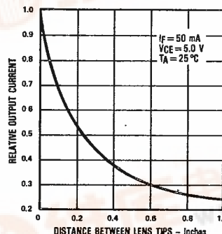
Coupling Characteristics of OP160SL and OP500
