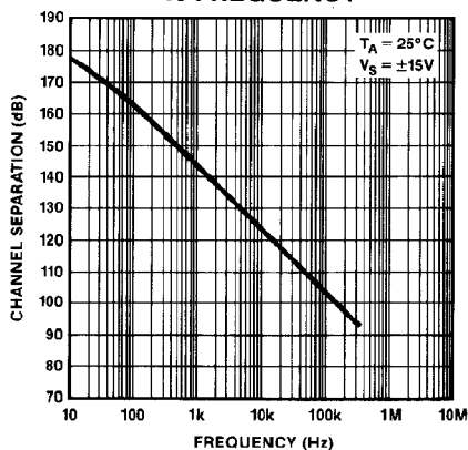
CHANNEL SEPERATION vs FREQUENCY
