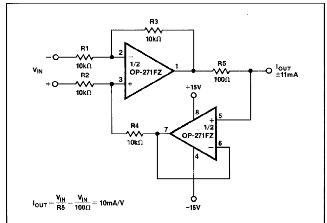
FIGURE 6: Fast Current Pump
