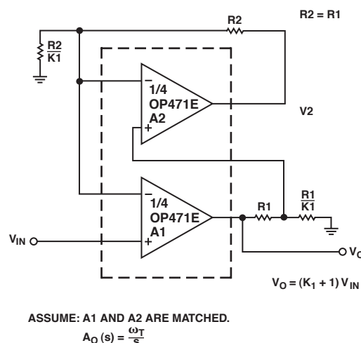
Figure 18. Low Phase Error Amplifier
