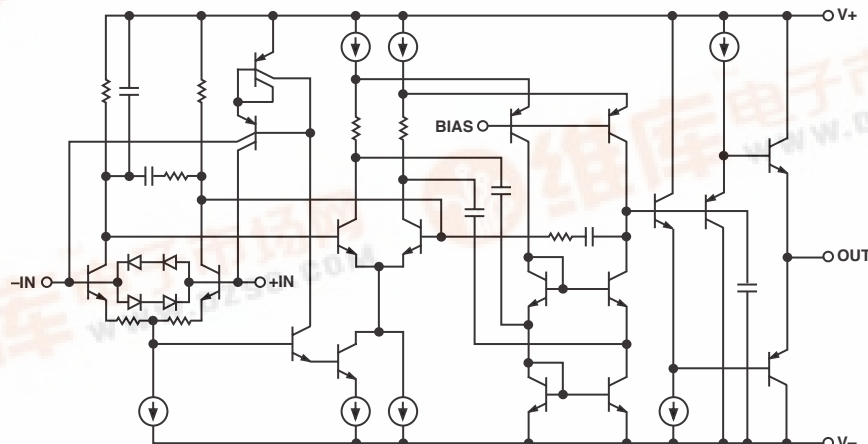
Figure 1. Simplified Schematic
