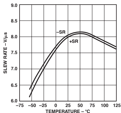
TPC 22. Slew Rate vs. Temperature
