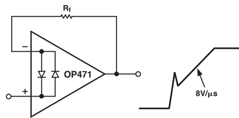
Figure 12. Pulsed Operation
