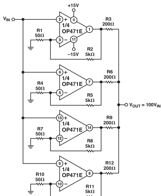
Figure 13. Low-Noise Amplifier
