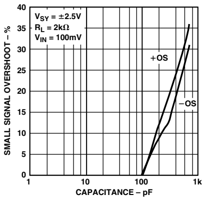
TPC 25. Small Signal Overshoot vs. Load Capacitance
