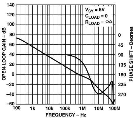
TPC 16. Open Loop Gain and Phase Shift vs. Frequency
