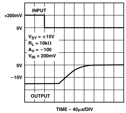
TPC 27. Negative Overtolerance Recovery
