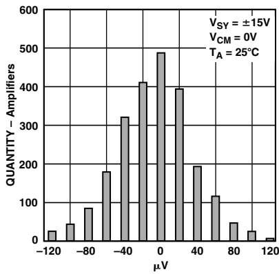
TPC 5. OP747 Input Offset Voltage Distribution
