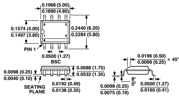
8-Pin SOIC (SO-8)
