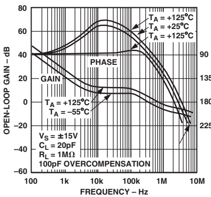
TPC 26. Open-Loop Gain, Phase vs. Frequency ( C_{OC} = 10,000 pF)
