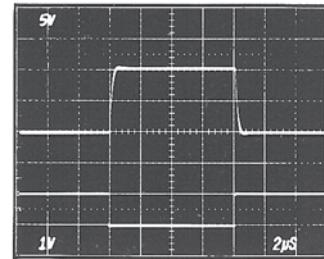
Figure 12. Combination Amplifier Transient Response
