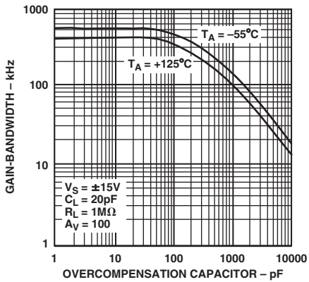
TPC 24. Gain Bandwidth Product vs. Overcompensation
