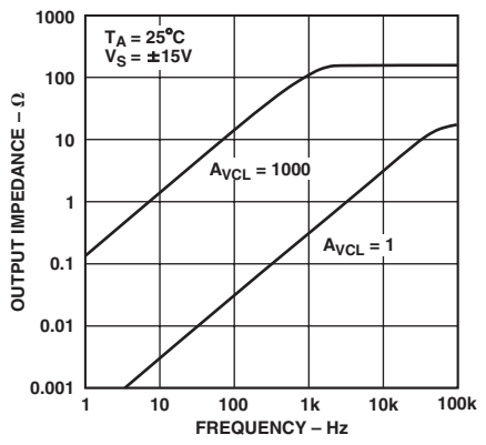
TPC 27. Closed-Loop Output Resistance vs. Frequency
