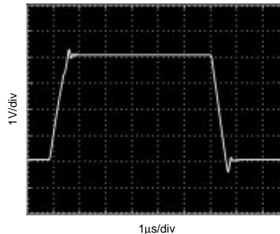
LARGE-SIGNAL STEP RESPONSE C_L = 100\text{pF}
