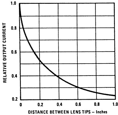
Coupling Characteristics of OP165 and OP505
