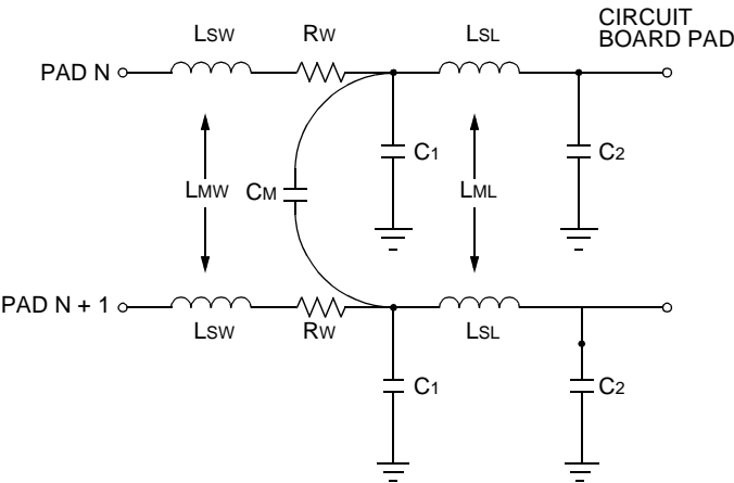
Figure 25. Package Parasitics
