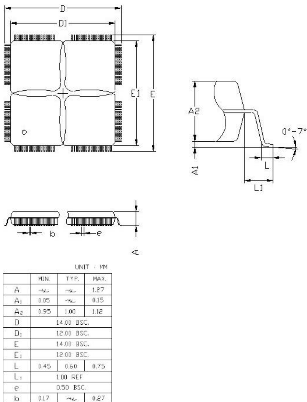
Figure 9: 68 Pin Plastic Leaded Chip Carrier
