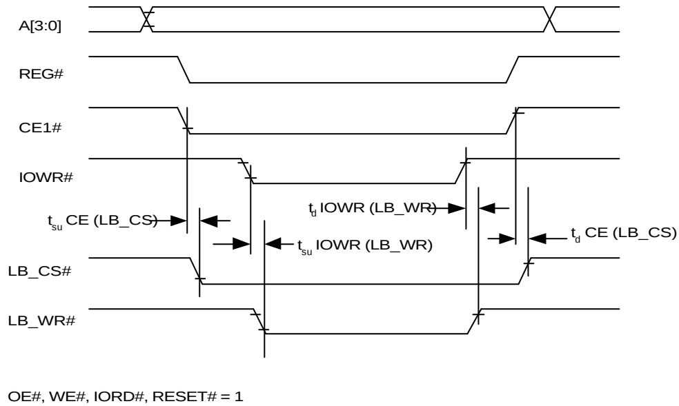
Figure 12: Local Bus write timing
