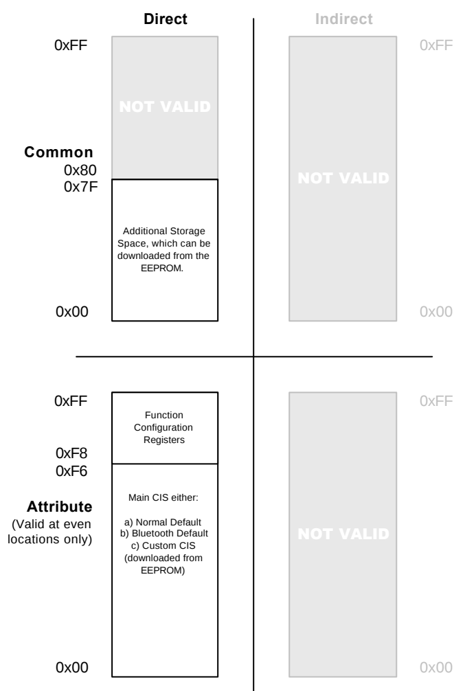
Figure 4: Normal Mode memory space map
