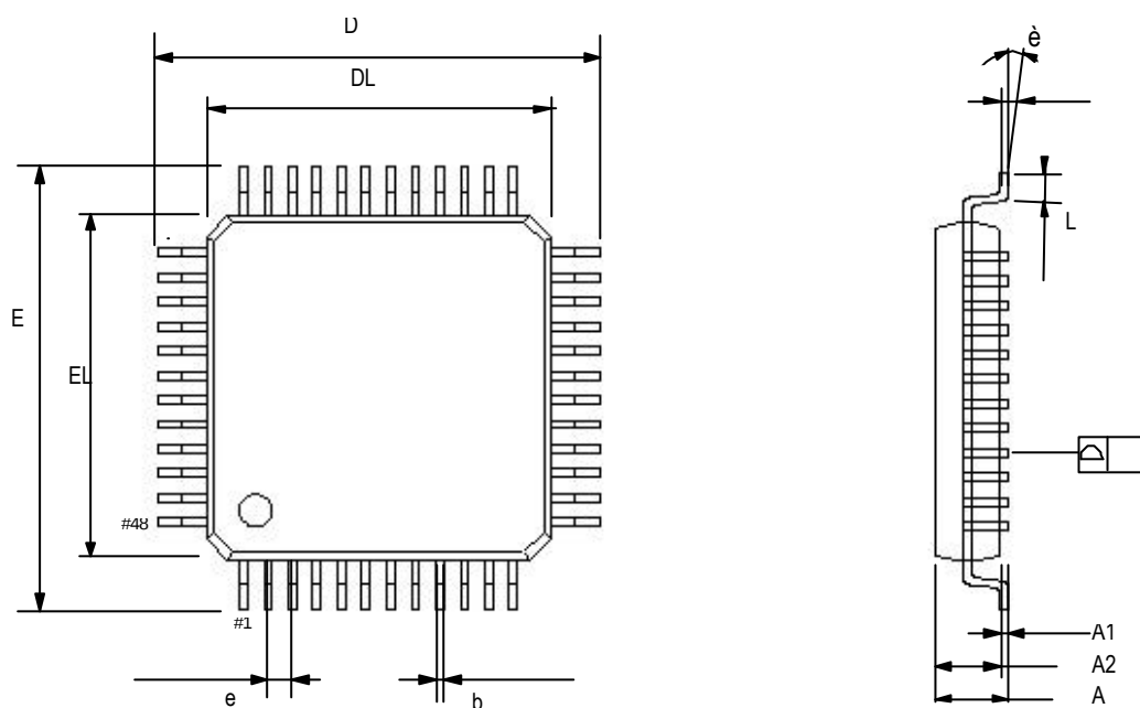
Figure 13: Device packaging
