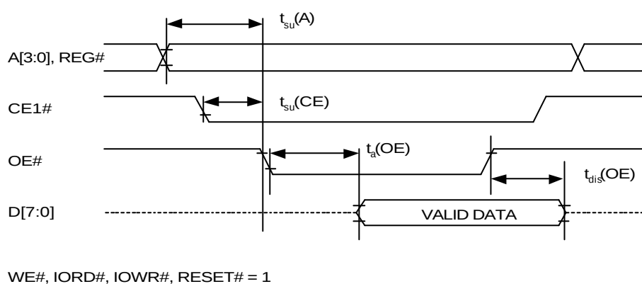
Figure 7: Common Memory Read Timing
