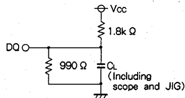
Fig.1 Output load
