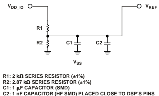
Figure 6. V_{REF} Filtering Scheme
