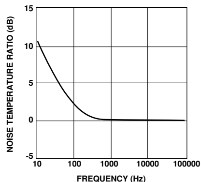
Figure 14. Typical Noise Temperature Ratio.
