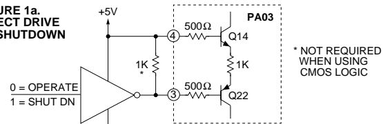
FIGURE 1b. HIGH VOLTAGE LOGIC INTERFACE
