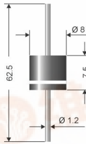
Axial lead diode
