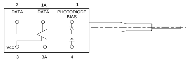
Figure 2. P171-Type R-PAK PIN/Preamp with Optional Differential Output Schematic (Top View)
