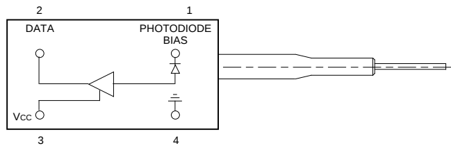
Figure 1. P171-Type R-PAK PIN/Preamp Schematic (Top View)
