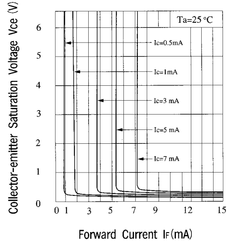
Fig. 9 Collector-emitter Saturation Voltage vs. Forward Current
