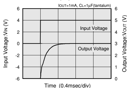
XC62FP3002 (3V)
