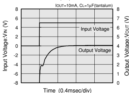
XC62FP4002 (4V)
