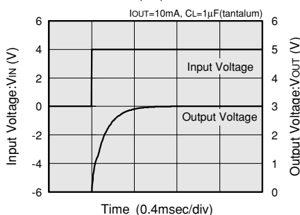
XC62FP3002 (3V)
