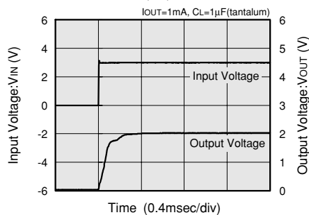
XC62FP2002 (2V)
