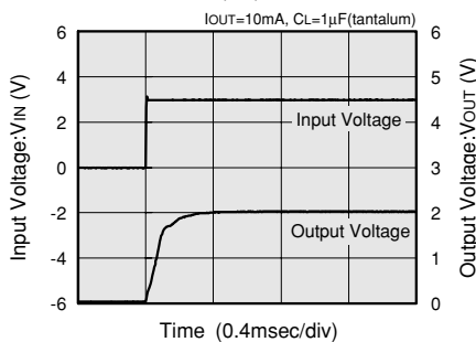
XC62FP2002 (2V)
