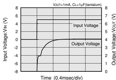
XC62FP4002 (4V)
