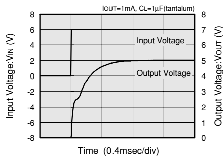
XC62FP5002 (5V)
