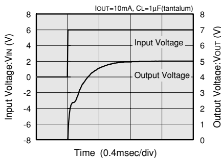
XC62FP5002 (5V)
