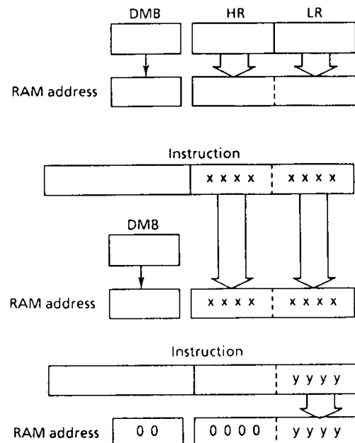
Figure 2-5. Addressing mode
