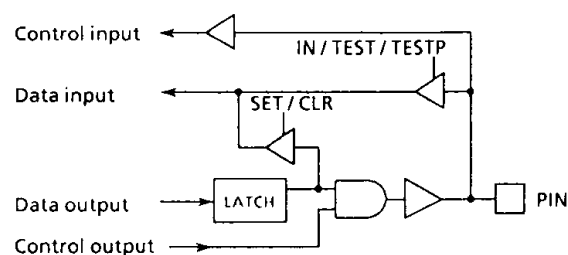
Figure 3-10. Port R9
