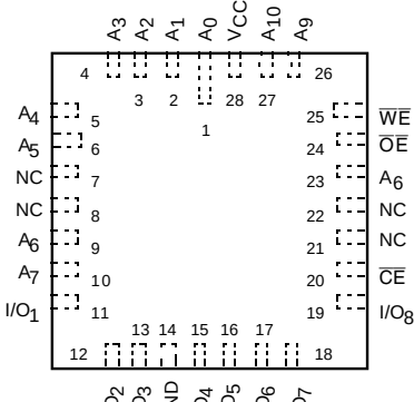
LCC (L5-1) TOP VIEW
