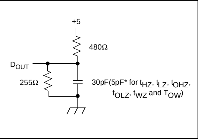
Figure 1. Output Load
