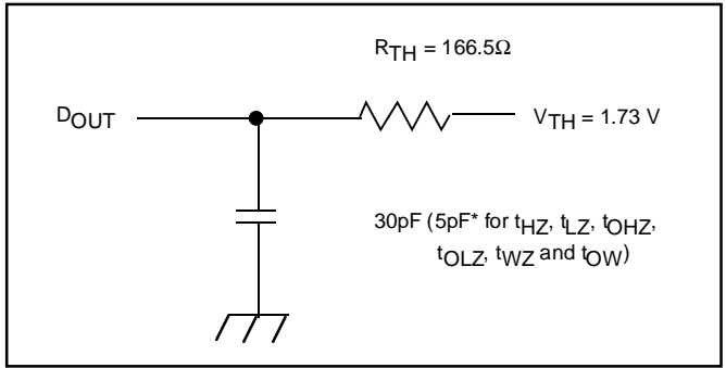
Figure 2. Thevenin Equivalent
