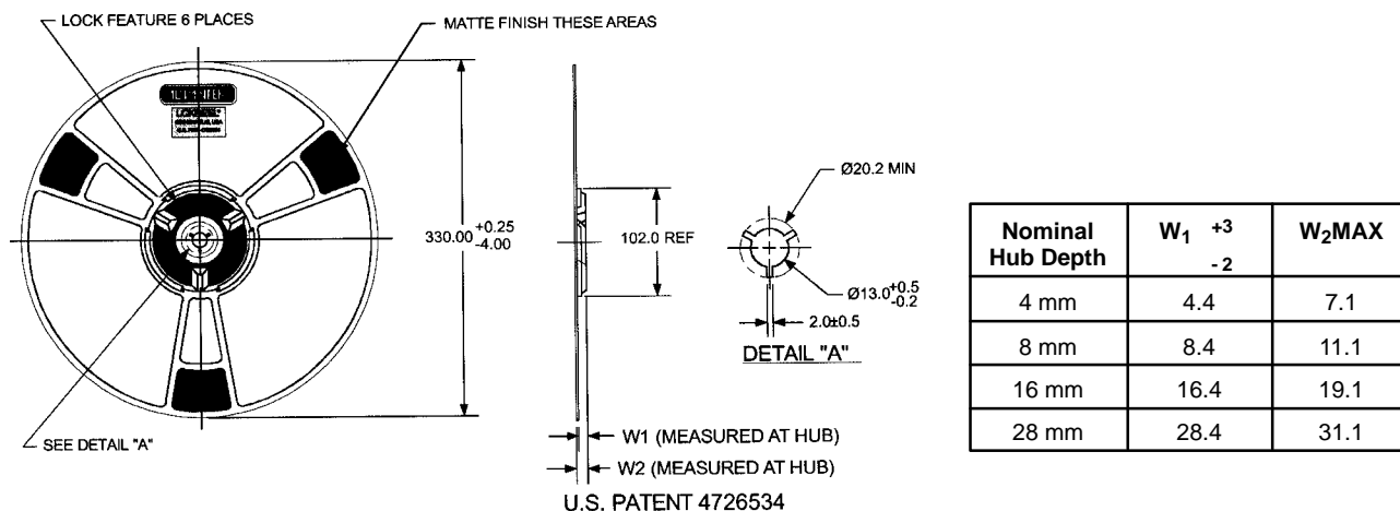
Figure 15. Reel Dimensions
