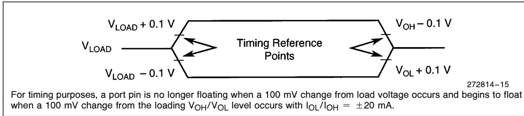
Figure 15. Float Waveforms
