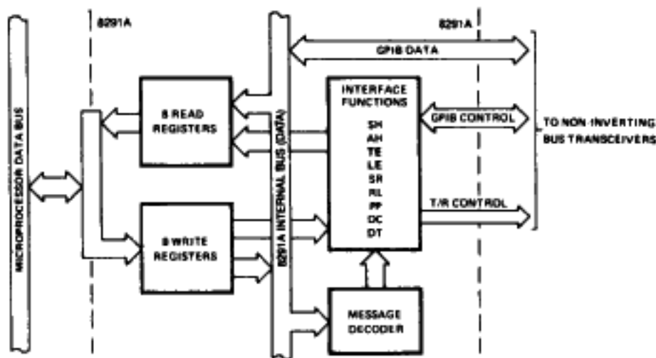
Figure 1. Block Diagram
