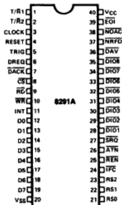
Figure 2. Pin Configuration
