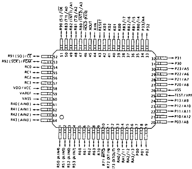
QFP64
