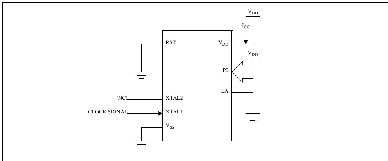
Figure 14: I_{CC} Test Condition, Idle Mode (All other pins are disconnected)
