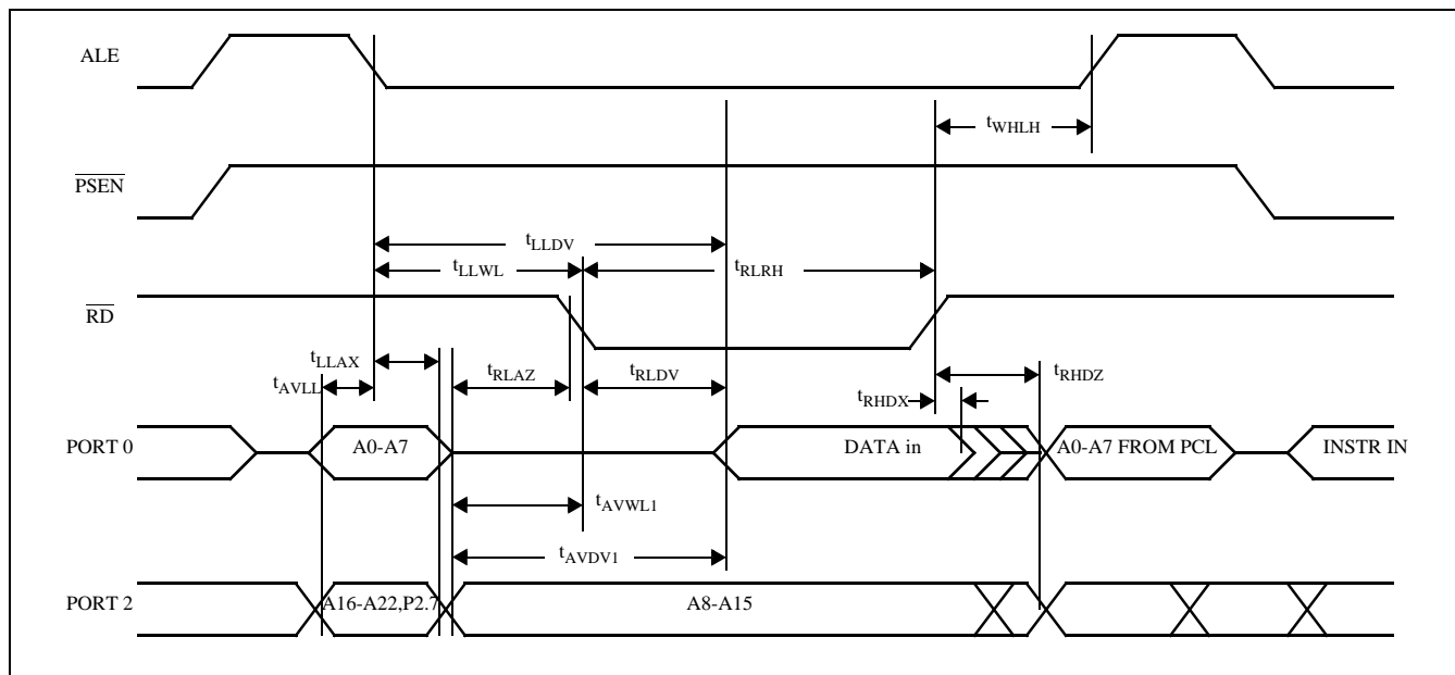
Figure 4: External Data Memory Read Cycle (Extended Memory Cycle)
