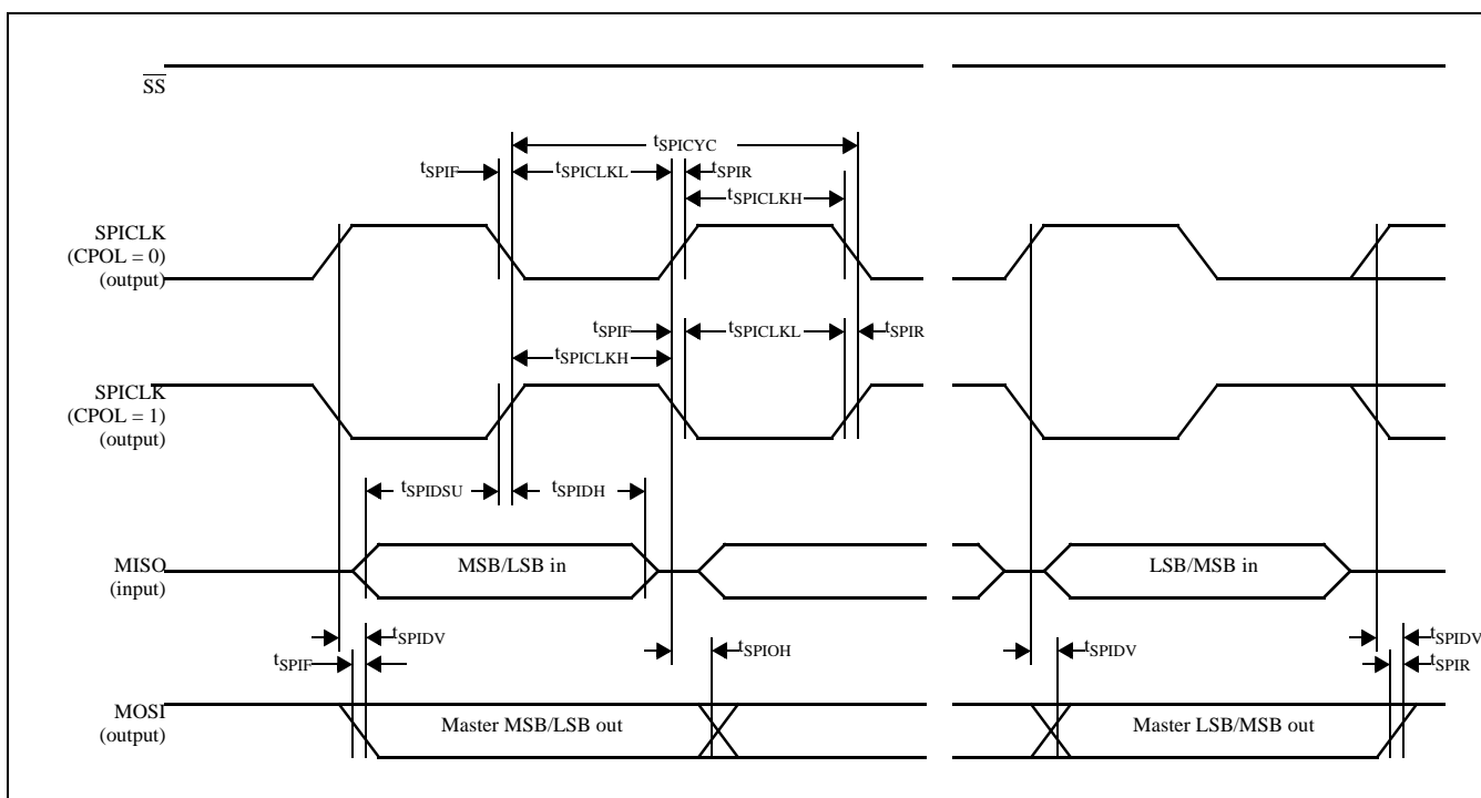
Figure 9: SPI Master Timing (CPHA = 1)
