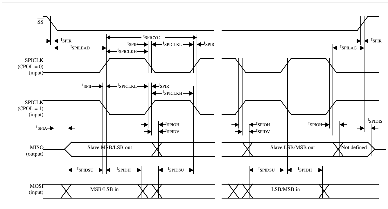
Figure 10: SPI Slave Timing (CPHA = 0)
