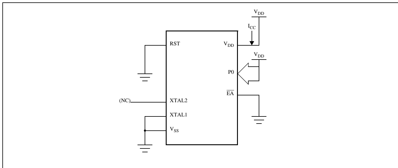
Figure 16: I_{CC} Test Condition, Power Down Mode (All other pins are disconnected, V_{DD} = 2.0V to 5.5V )
