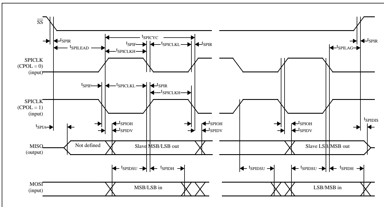
Figure 11: SPI Slave Timing (CPHA = 1)
