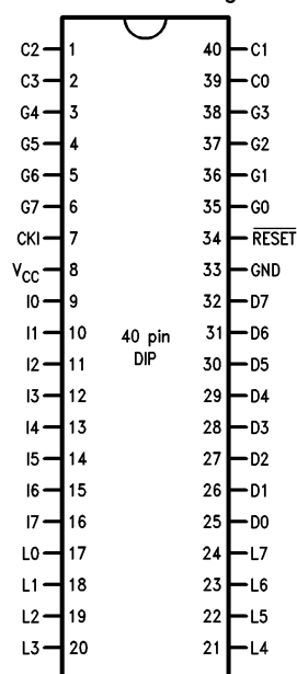
Dual-In-Line Package
