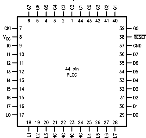
Plastic Chip Carrier
