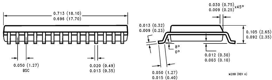
Small Outline Molded Dual-In-Line Package (M) Order Number COP881C-XXX/WM, COP981C-XXX/WM, COP681C-XXX/WM or COP981CH-XXX/WM NS Package Number M28B
