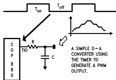
FIGURE 11. Timer Application
