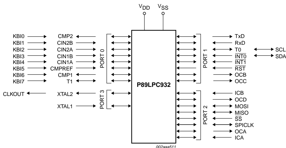
Fig 5. Logic symbol.
