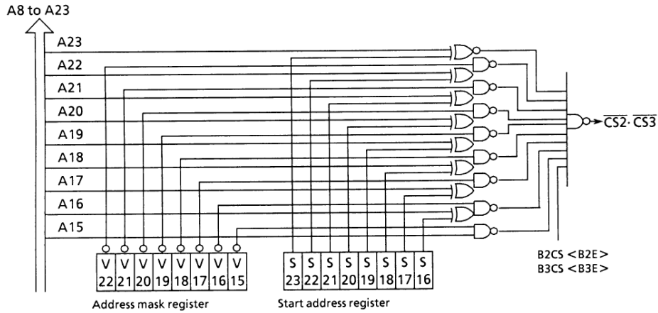
Figure 3.6 (4). CS1 Address Decode Block Diagram
