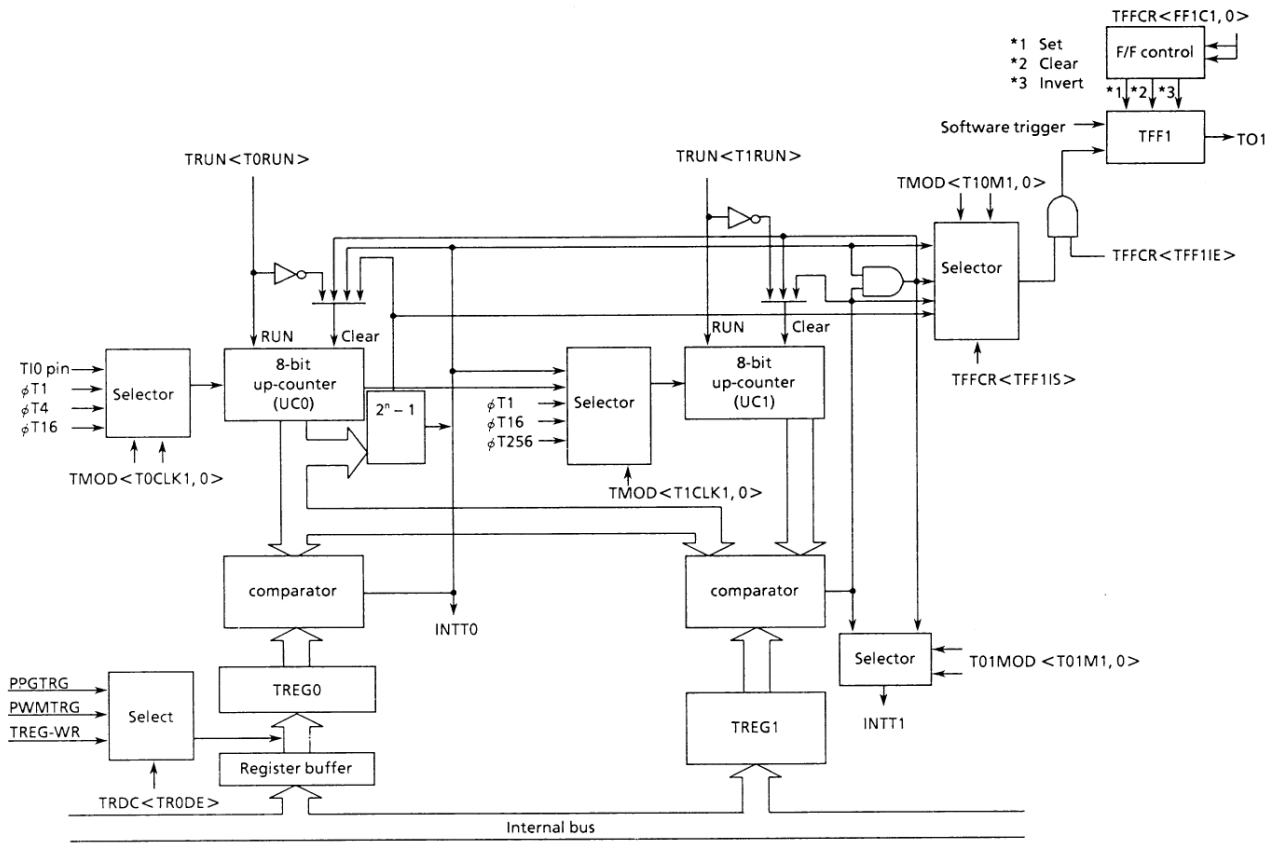
Figure 3.8 (1). Block Diagram of 8-bit Timers (Timers 0 and 1)
