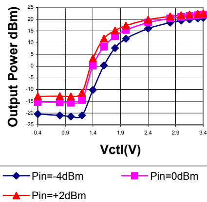
Output Power vs Control Voltage
