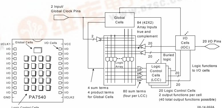
Figure 2. Block Diagram
