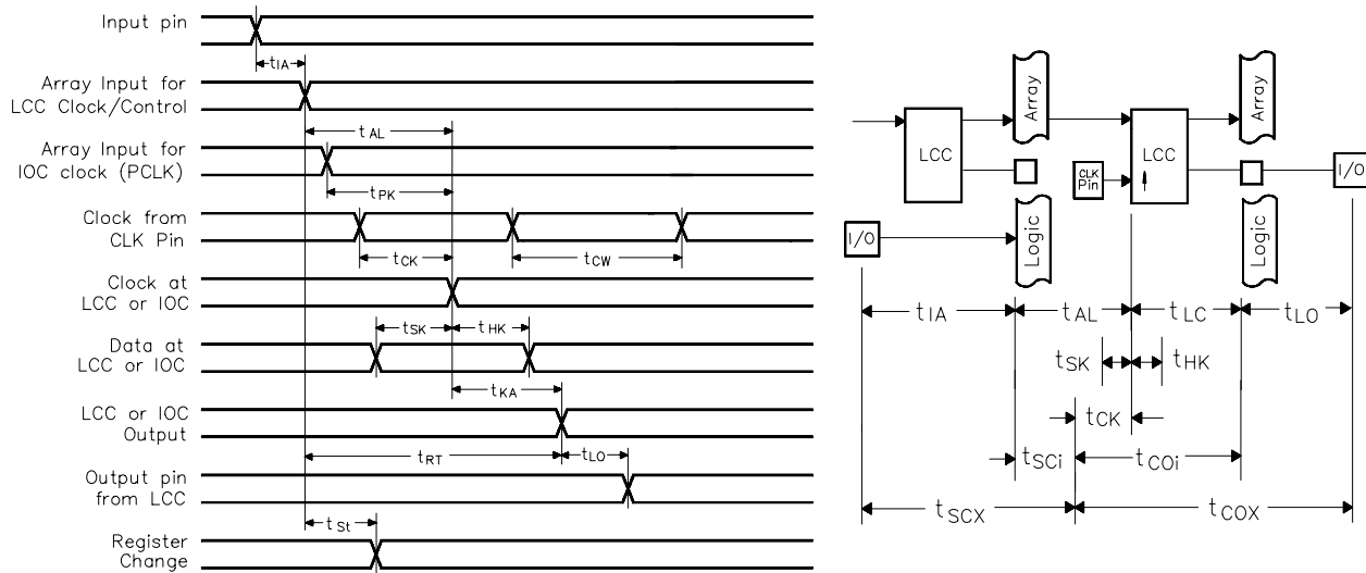
Figure 15. Sequential Timing – Waveforms and Block Diagram
