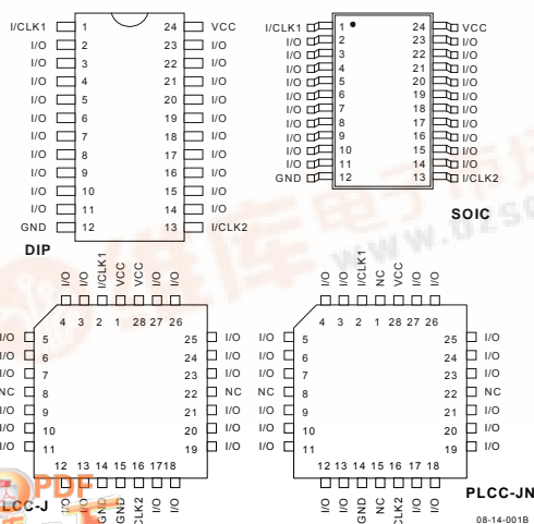
Figure 1. Pin Configuration
