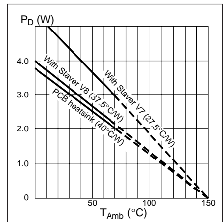
Figure 13. Allowable power dissipation vs. ambient temperature.
