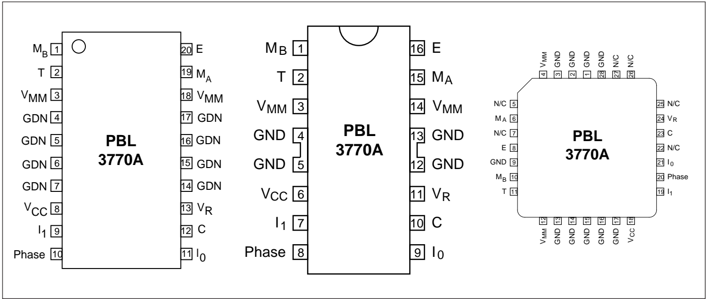
Figure 3. Pin configurations.
