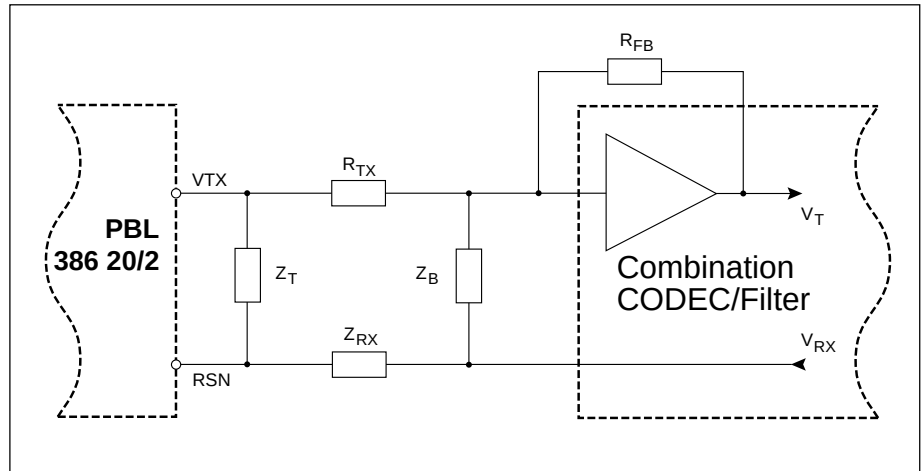
Figure 10. Hybrid function.
