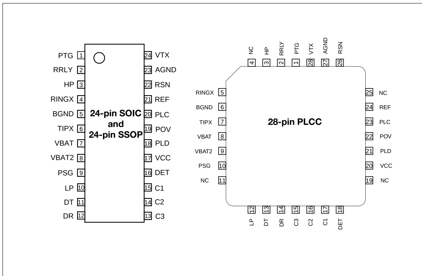
Figure 8. Pin configuration, 24-pin SSOP, 24-pin SOIC and 28 pin PLCC package, top view.
