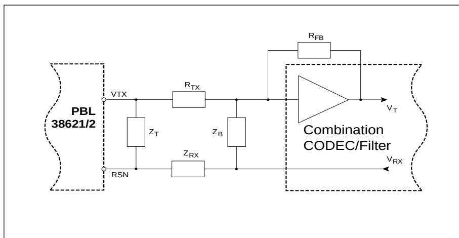
Figure 9. Hybrid function.
