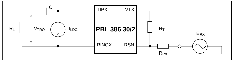
Figure 2. Overload level, V_{\text{TRO}} , two-wire port
