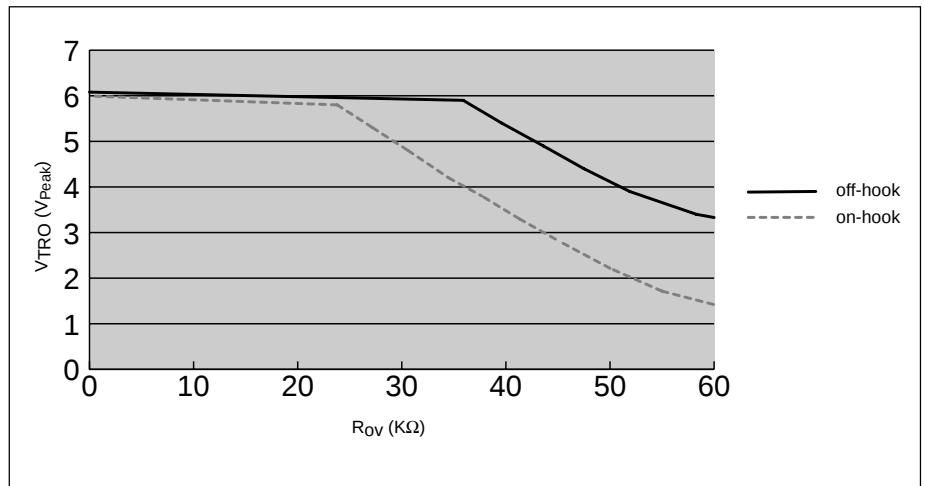
Figure 10. Programmable overhead voltage (POV). R_{\text{L}} = 600 \Omega or \infty .
