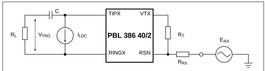
Figure 2. Overhead voltage, V_{\text{TRO}} , two-wire port
