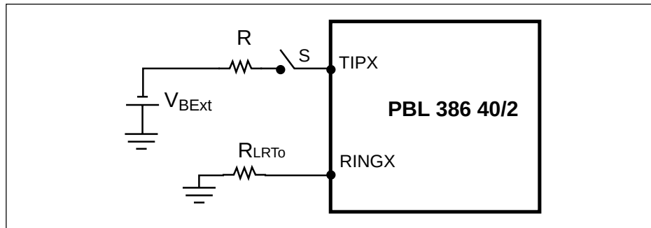
Figure 7. Tipx voltage.
