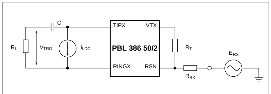
Figure 2. Overhead voltage, V_{\text{TRO}} , two-wire port
