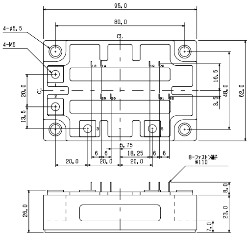
OUTLINE DRAWING
