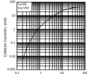
Collector Current vs. Forward Current
