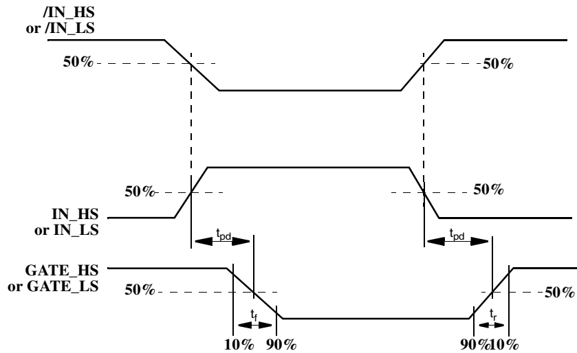
Figure 3. Dynamic Characteristics
