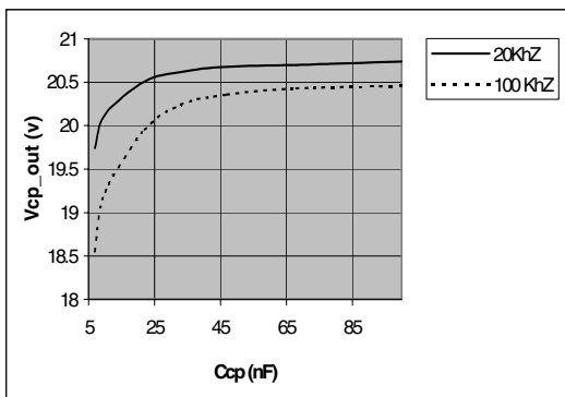
MTP60N06HD (Q g =50nC)
