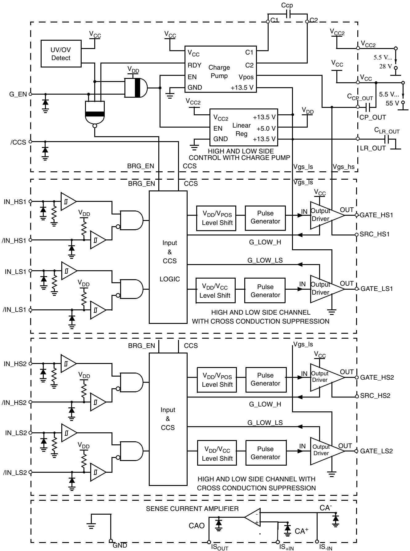
MC33253 Figure 1. Principal Building Blocks
