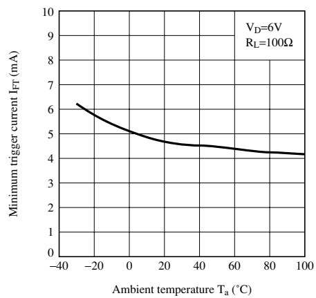
Fig.4 Minimum Trigger Current vs. Ambient Temperature
