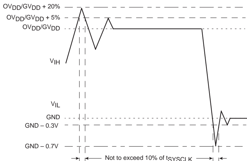
Figure 3. Overshoot/Undershoot Voltage
