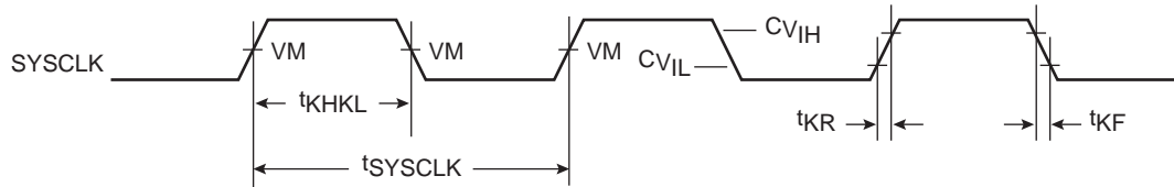
Figure 8. SYCLK Input Timing Diagram
