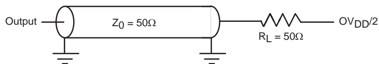
Figure 18. Alternate AC Test Load for the JTAG Interface
