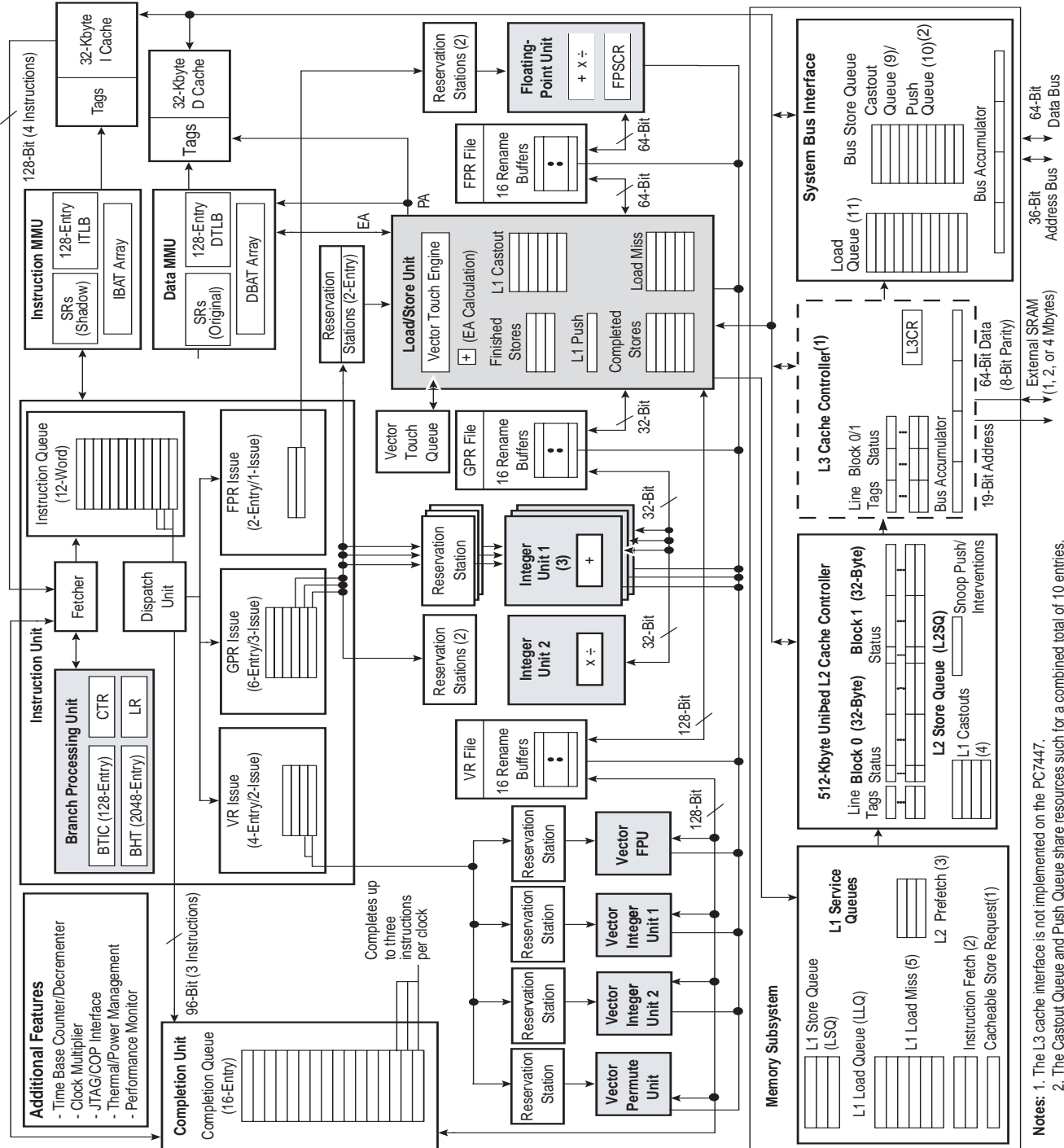
Figure 1. PC7457 Microprocessor Block Diagram
