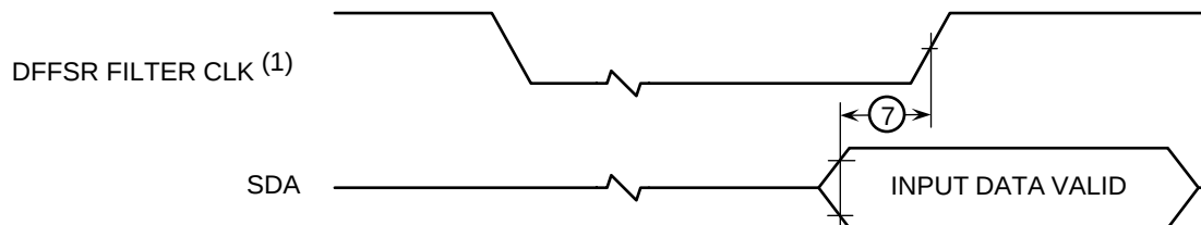
Figure 17. Two-wire Interface Timing Diagram III
