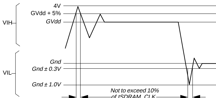
Figure 3. Overshoot/Undershoot Voltage
