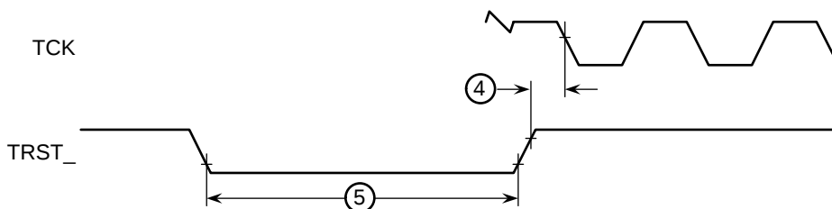
Figure 22. JTAG TRST Timing Diagram
