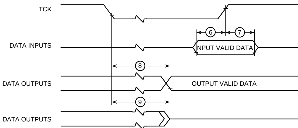
Figure 23. JTAG Boundary Scan Timing Diagram
