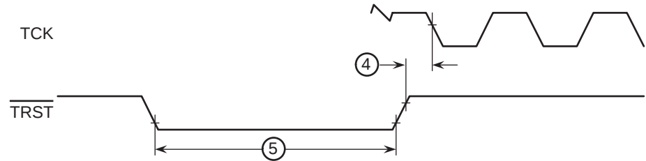
Figure 25. JTAG \overline{\text{TRST}} Timing Diagram
