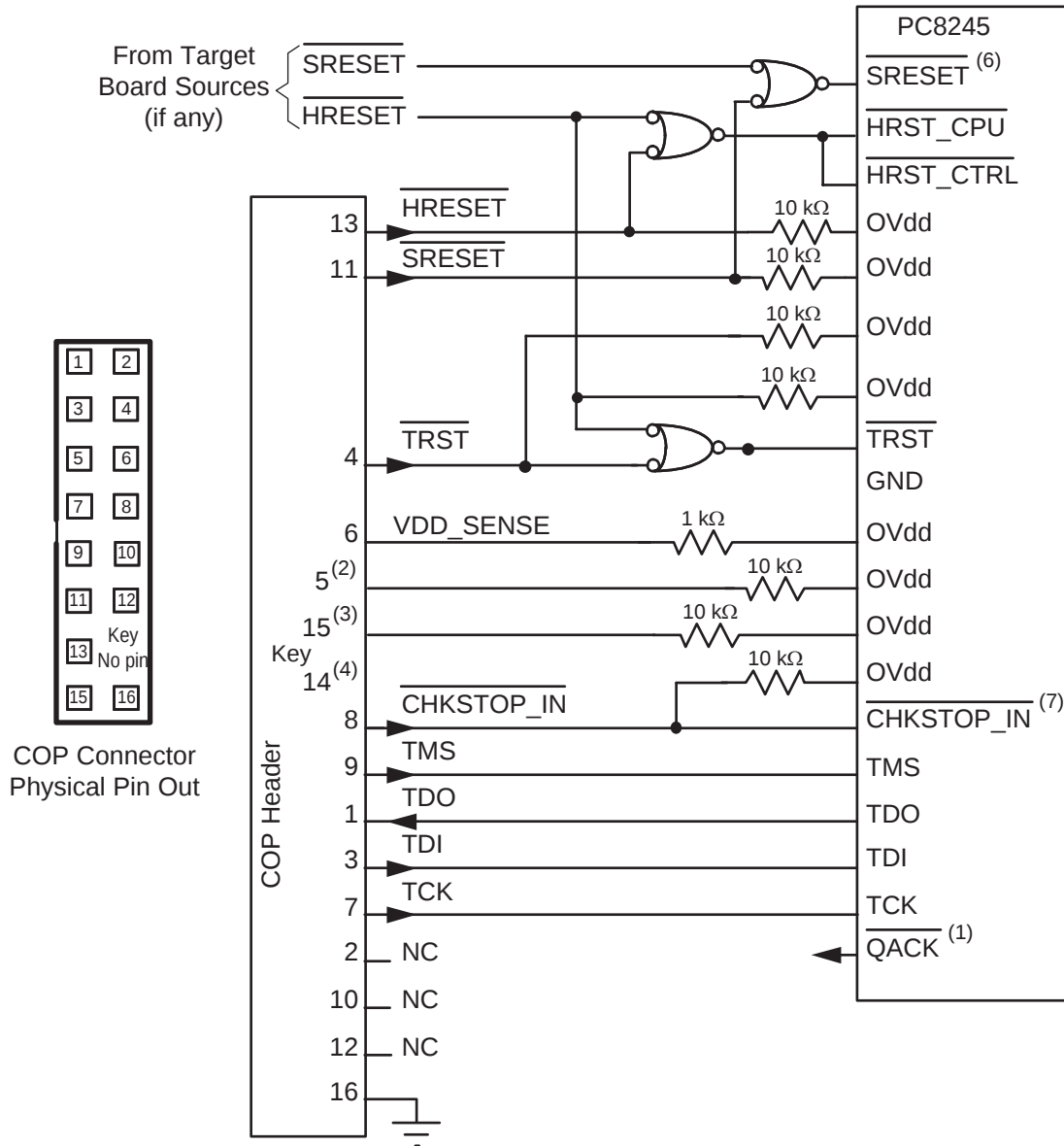
Figure 30. COP Connector Diagram
