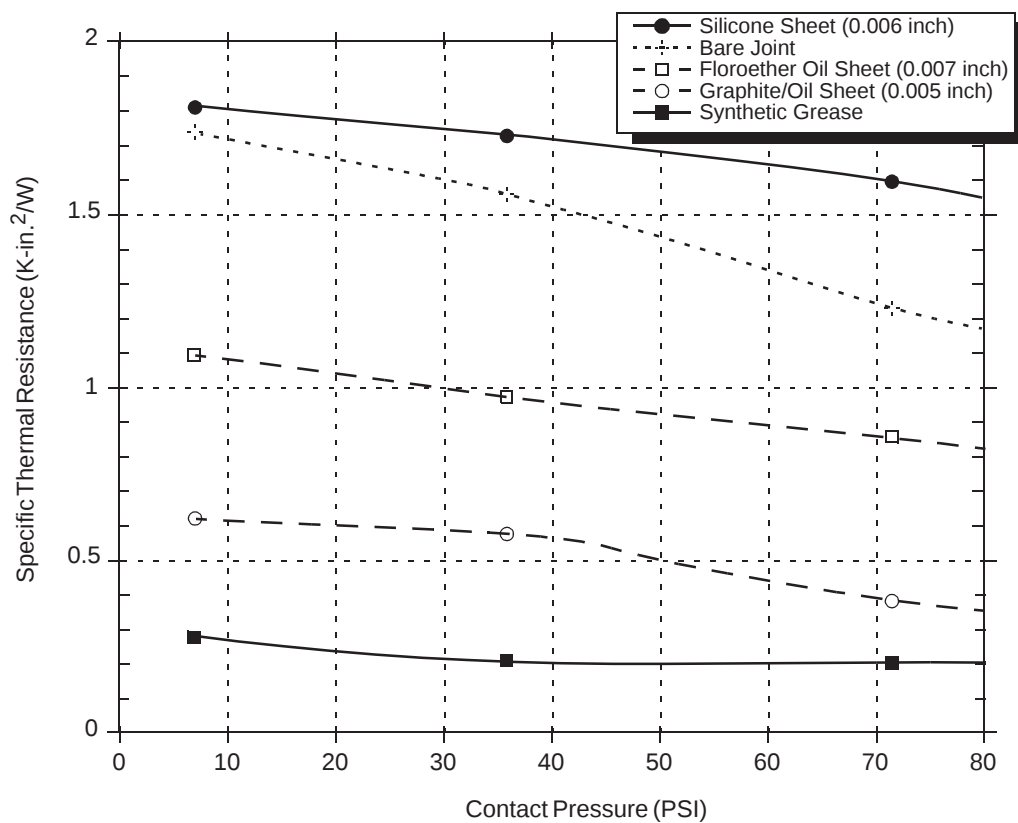
Figure 7. Thermal Performance of Select Thermal Interface Material
