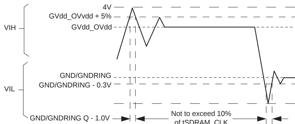
Figure 3. Overshoot/Undershoot Voltage
