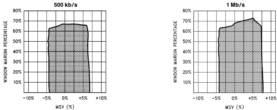
TL/F/11332-11 FIGURE 5-4. PC8477B Dynamic Window Margin Performance with \pm 3\% ISV at 1 kHz (Typical performance at V_{CC} = 5.0V , 25^{\circ}C )
