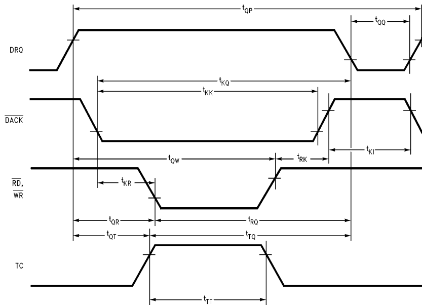
FIGURE 6-4. DMA Timing
