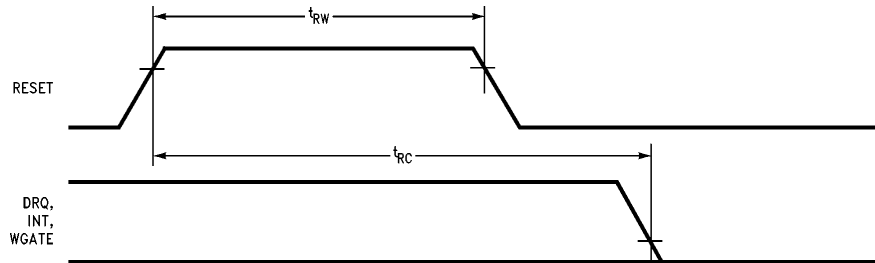
FIGURE 6-5. Reset Timing
